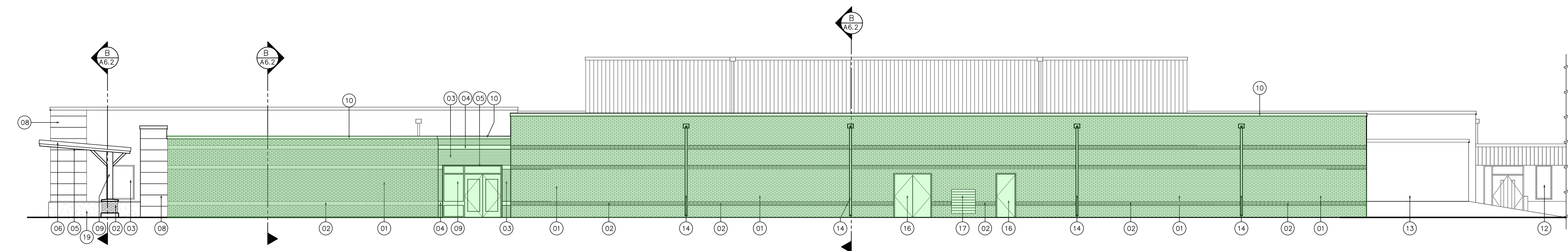
04 PARTIAL EAST ELEVATION SCALE: 1/8" = 1'-0"
