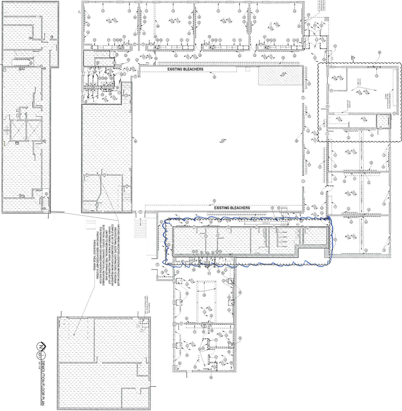
DEMOLITION PLAN - LOWER LEVEL
