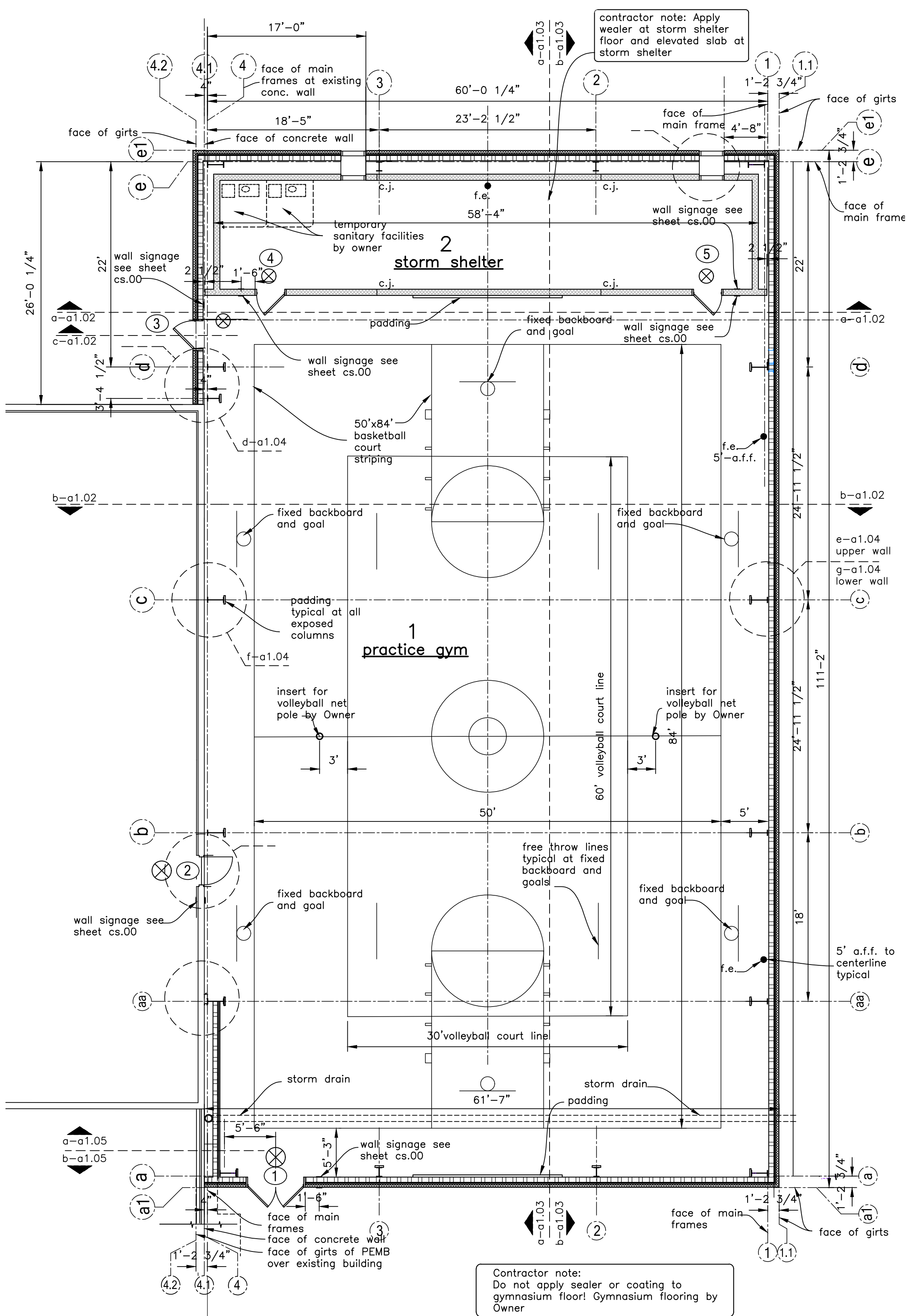
a floor plan 1/8" = 1'-0"
