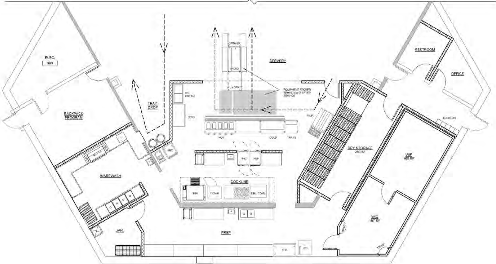
FOODSERVICE EQUIPMENT PLAN OPT B 1/4" = 1'-0"
