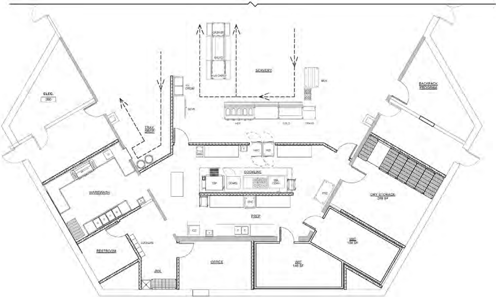
FOODSERVICE EQUIPMENT PLAN OPT A 1/4" = 1'-0"
