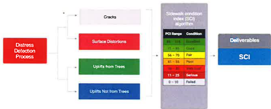
Sidewalk Algorithm
