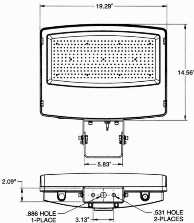
SGF3 (TRUNNION)
