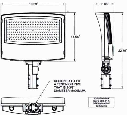
SGF3 (KNUCKLE)
