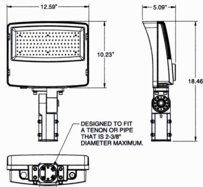
SGF2 (KNUCKLE)
