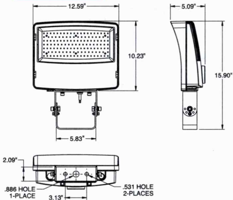
SGF2 (TRUNNION)
