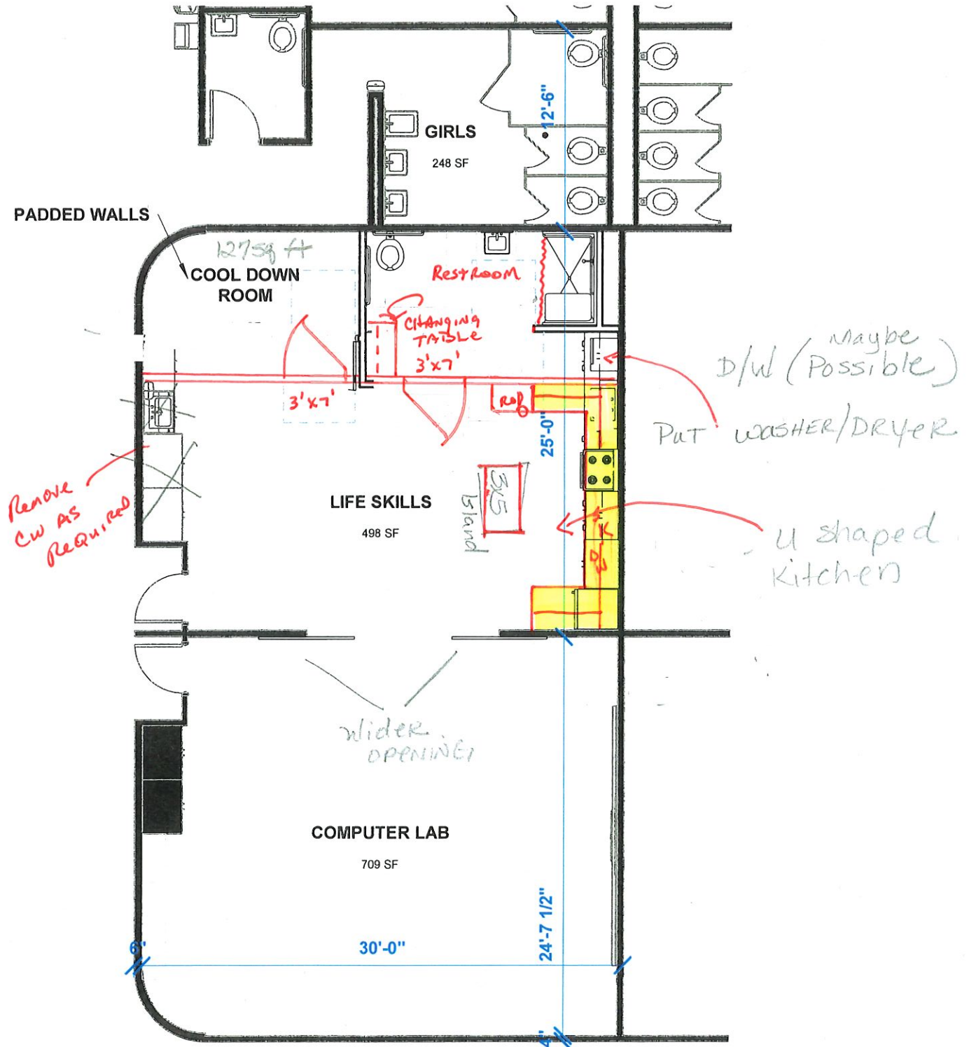
1 FLOOR PLAN "B" 1/8" = 1'-0"
