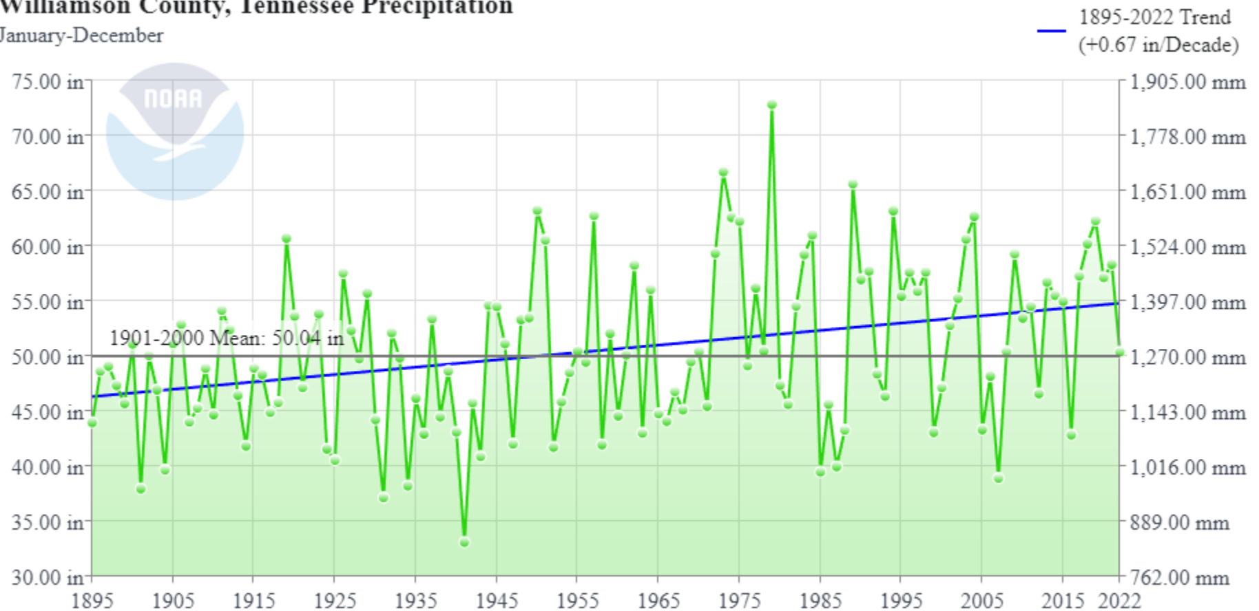
Figure 2: Total Annual Precipitation for Williamson County, Tennessee, Showing a +0.67-inch Increase per Decade Since 1895.
