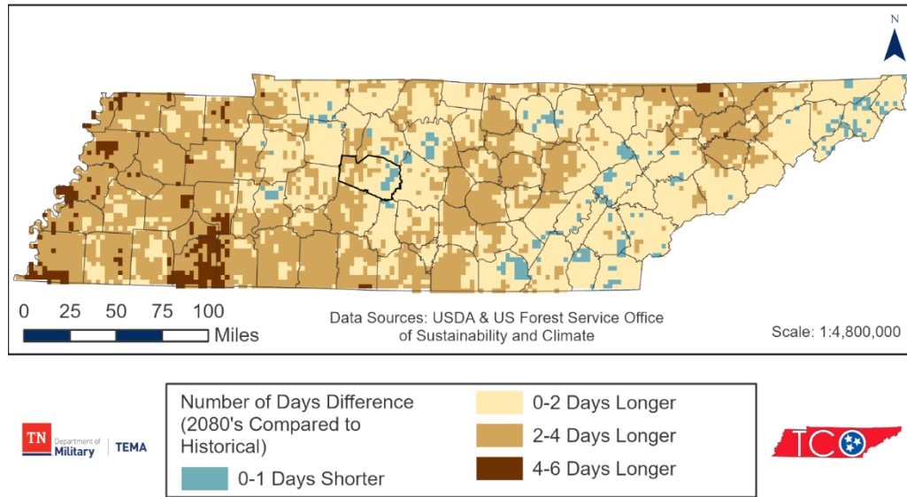
Figure 39: Change in the Length of a 10-Year (10% Annual Probability of Occurrence) Drought from Historical Data (1975-2005) to a 10-Year Drought in the 2080s (RCP8.5 Scenario), Williamson County Outlined in Bold.
