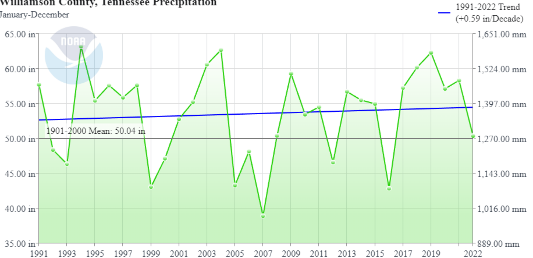
Figure 4: Total Annual Precipitation for Williamson County, Tennessee, Showing a +0.59-inch Increase per Decade Since 1991.
