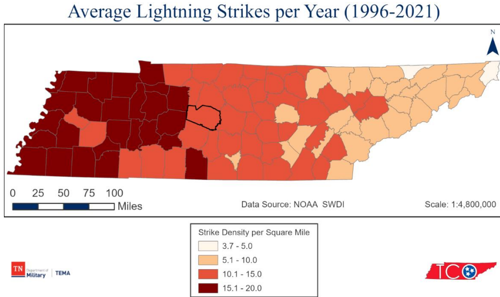
Figure 18: Average Annual Number of Lightning Strikes per Square Mile from 1996 to 2021, Williamson County Outlined in Bold.
