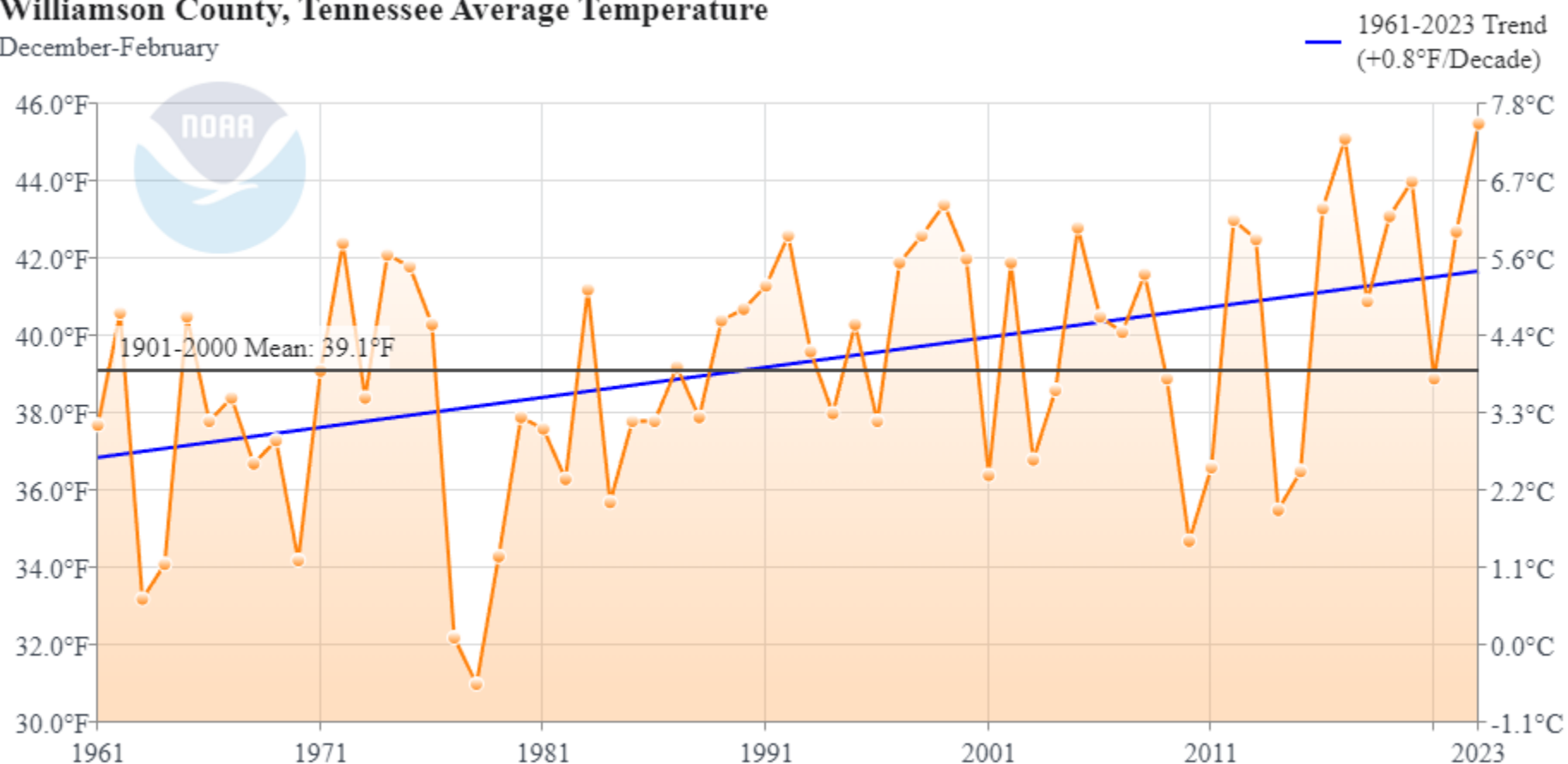
Figure 24: Winter (December to February) Mean Temperature for Williamson County, Tennessee, Showing a +0.8°F Increase per Decade Since 1961.
