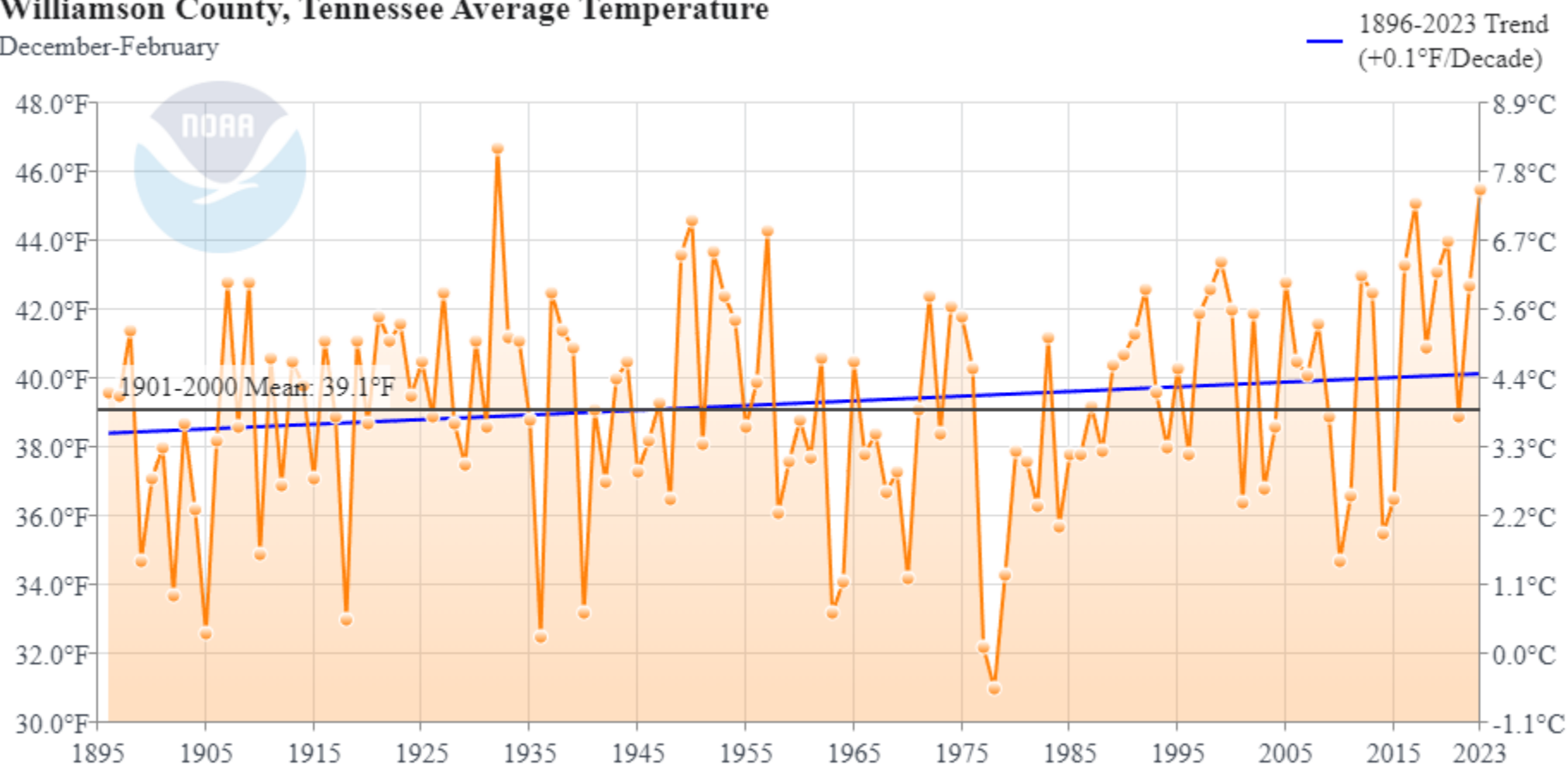
Figure 23: Winter (December to February) Mean Temperature for Williamson County, Tennessee, Showing a +0.1°F Increase per Decade Since 1895.
