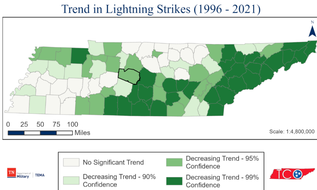
Figure 19: Trends in the Number of Lightning Strikes per County Recorded in the NOAA Severe Weather Data Inventory from 1996 to 2021, Williamson County Outlined in Bold.
