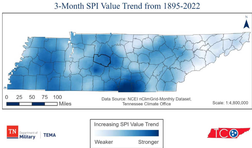
Figure 37: SPI Value Trend for 3-Months from 1895 to 2022, Williamson County Outlined in Bold.
