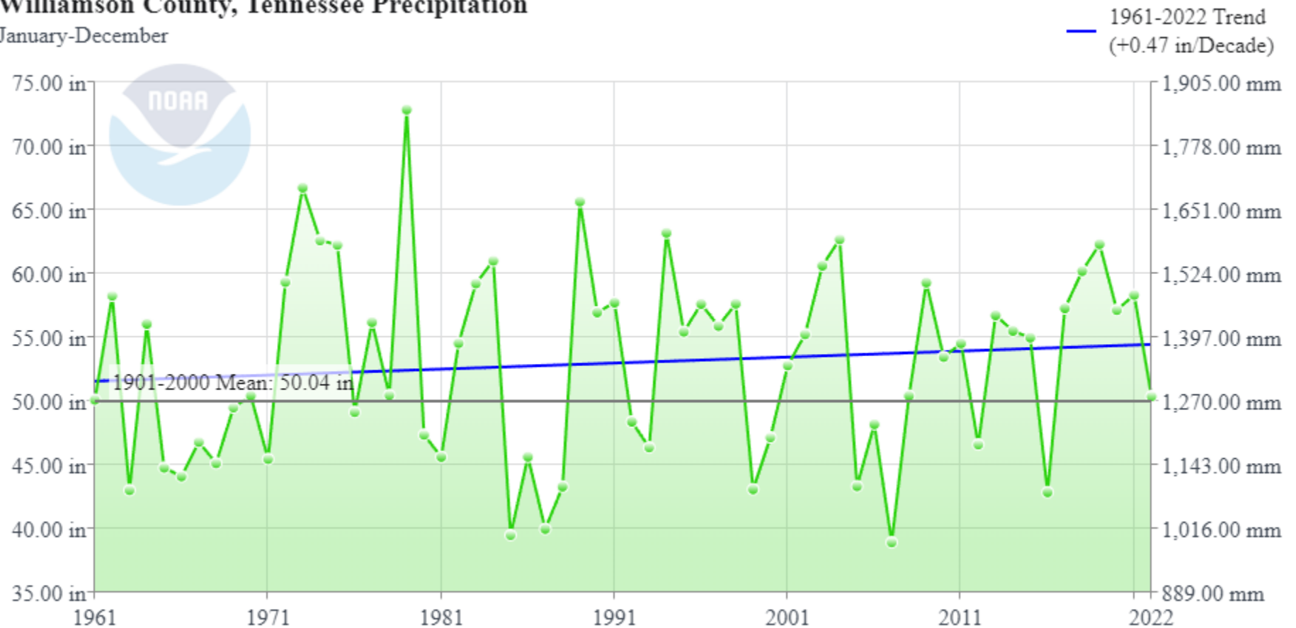
Figure 3: Total Annual Precipitation for Williamson County, Tennessee, Showing a +0.47-inch Increase per Decade Since 1961.
