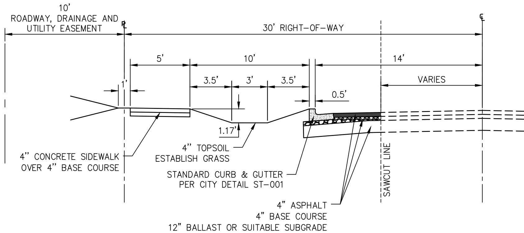
B MILES AVE AND MAPLE ST FRONTAGE IMPROVEMENTS
