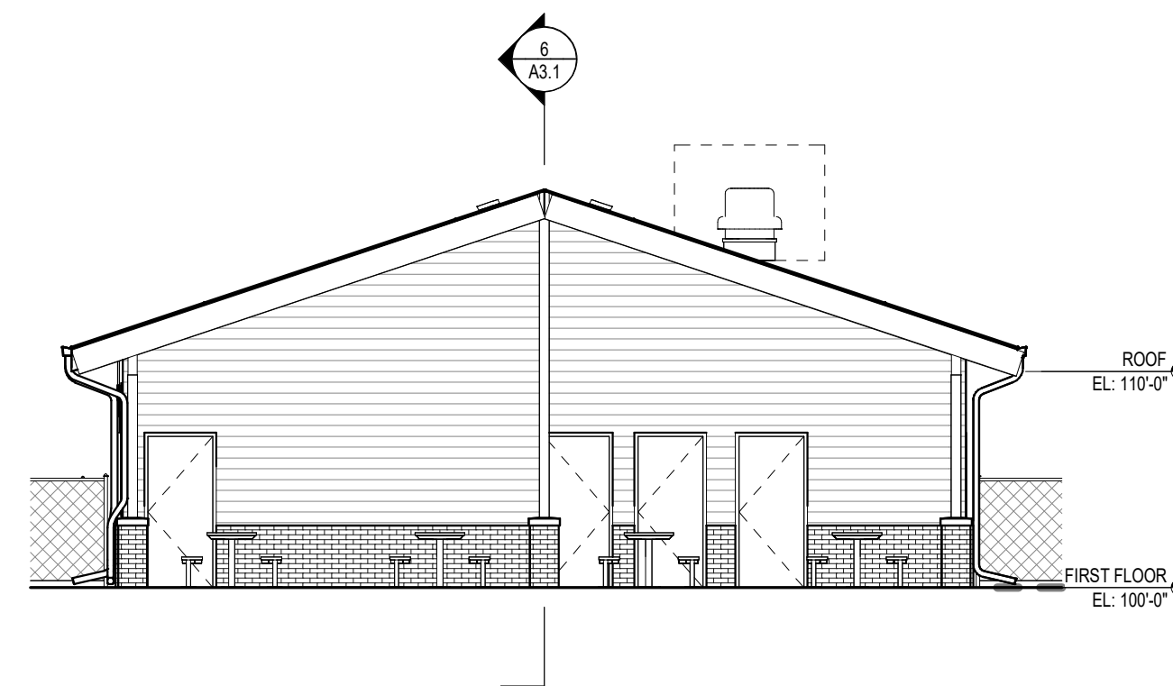
2 SOUTH ELEVATION A3.1 1/8" = 1'-0"
