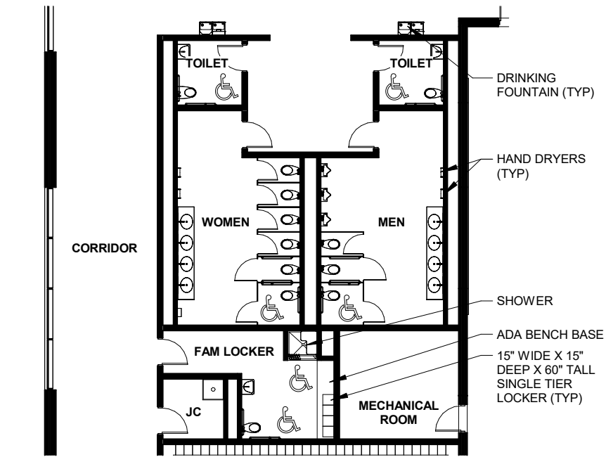
ENLARGED FLOOR PLAN - RESTROOMS 1/16" = 1'-0"
