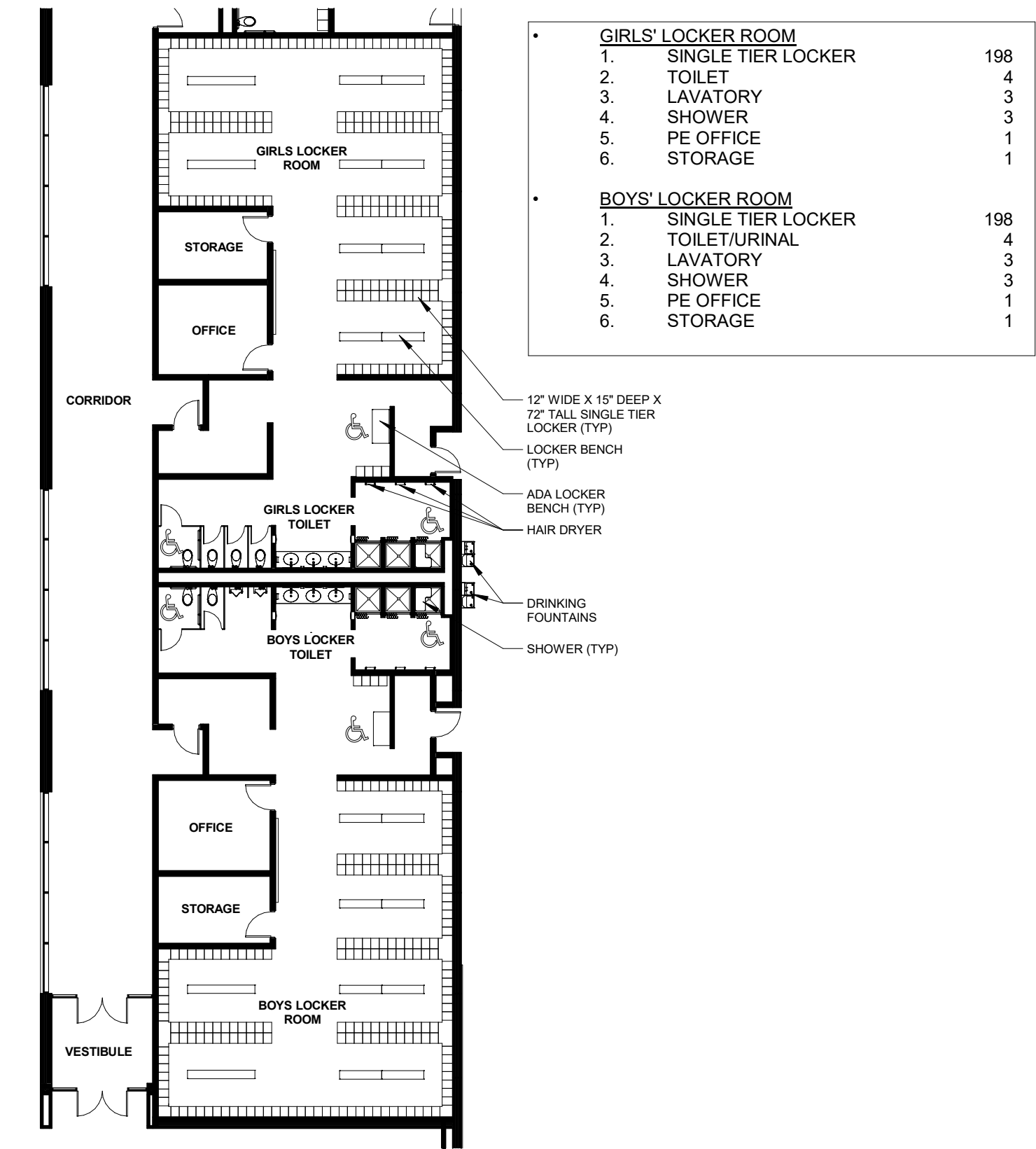
ENLARGED FLOOR PLAN - LOCKER ROOMS 1/16" = 1'-0"
