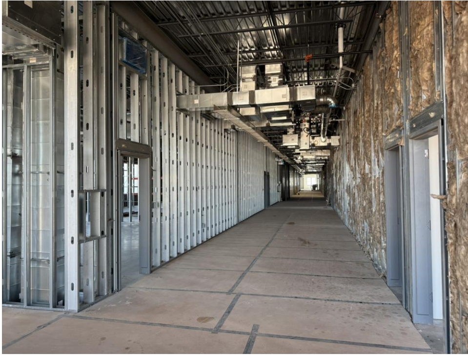
AREA 2 - HALLWAY 2 ND FLOOR
