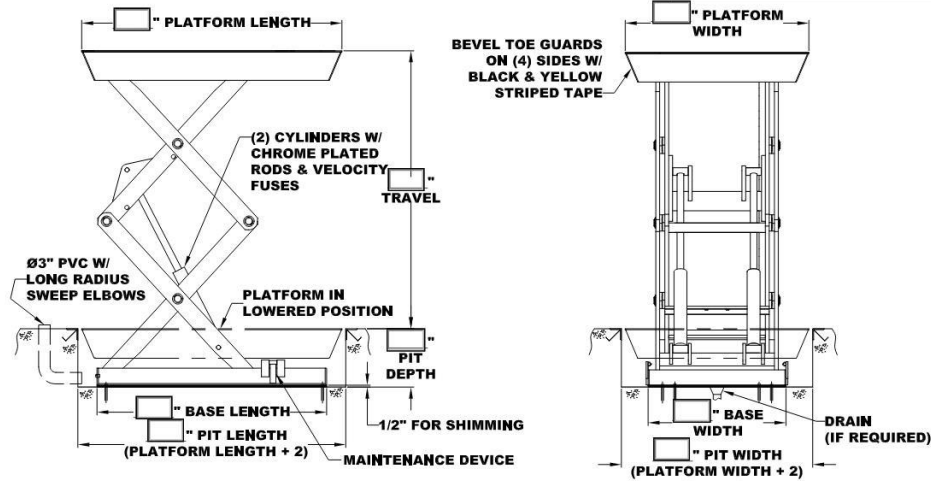
PIT MOUNTED DOUBLE PANTOGRAPH (DP) LIFT
