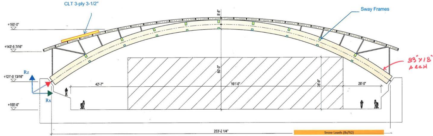
Reaction loads at piers (ADS loads)
